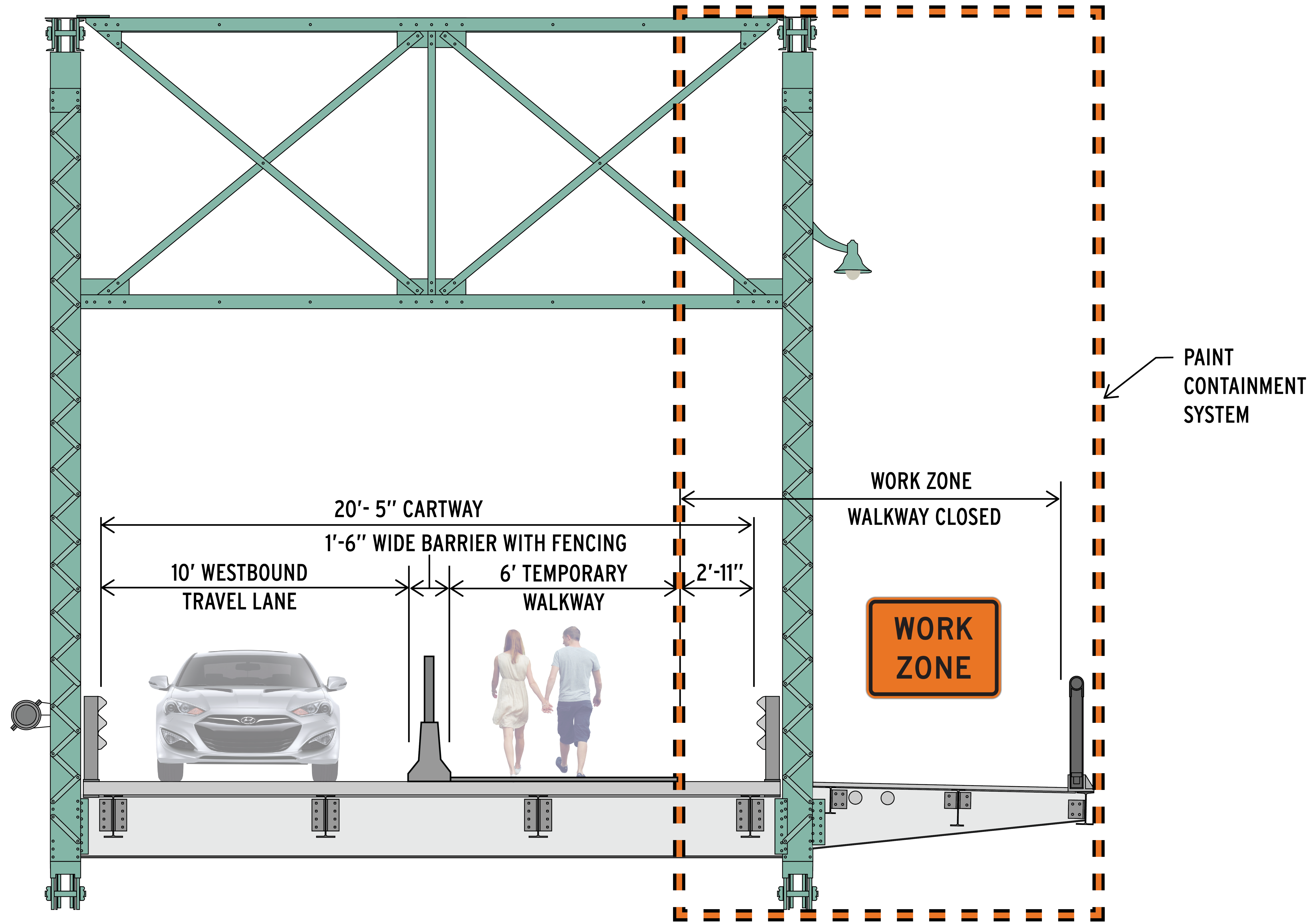
STAGE 3 - PORTION OF BRIDGE CLOSED (LOOKING EAST)
