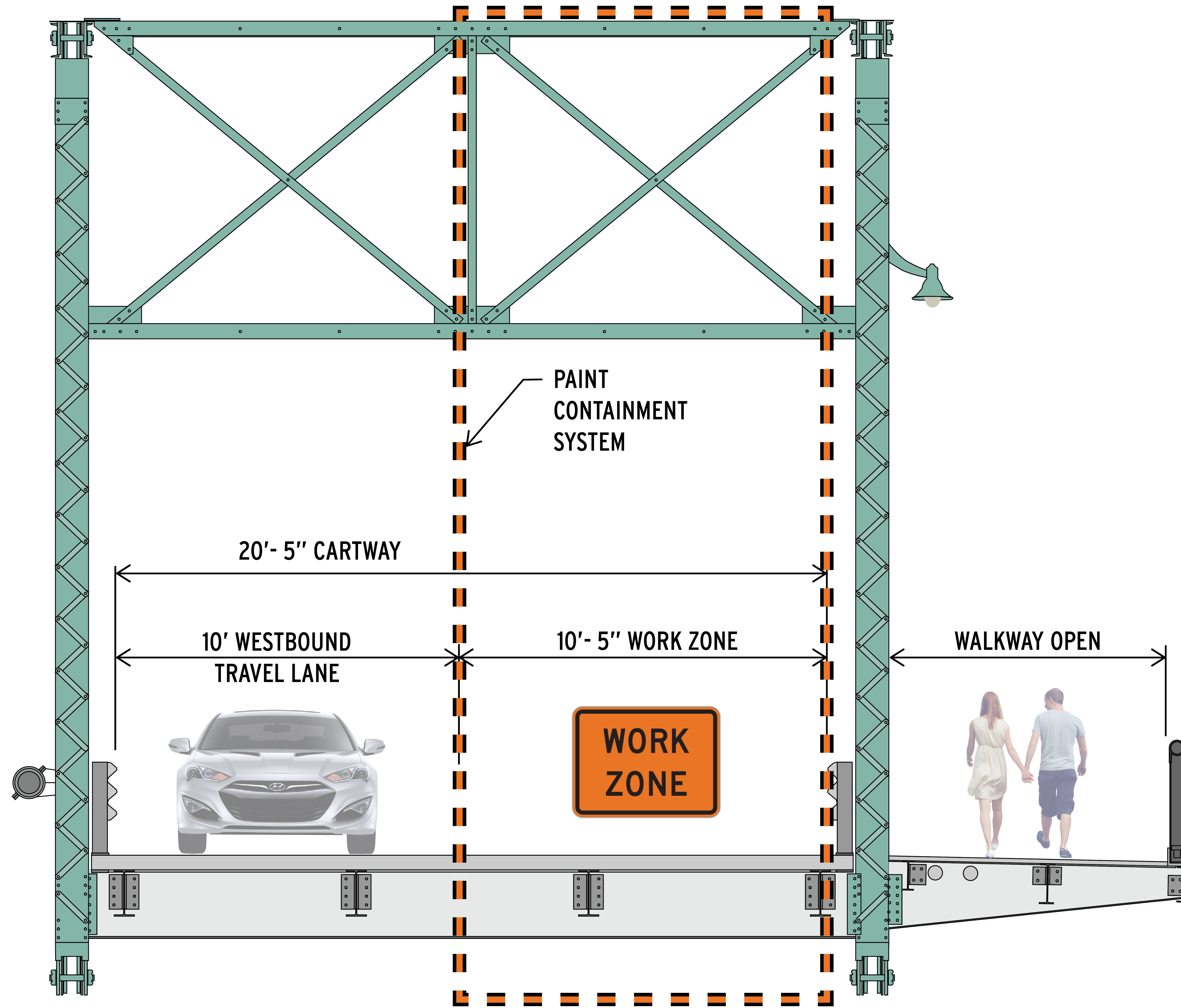
STAGE 2 - PORTION OF BRIDGE CLOSED (LOOKING EAST)
