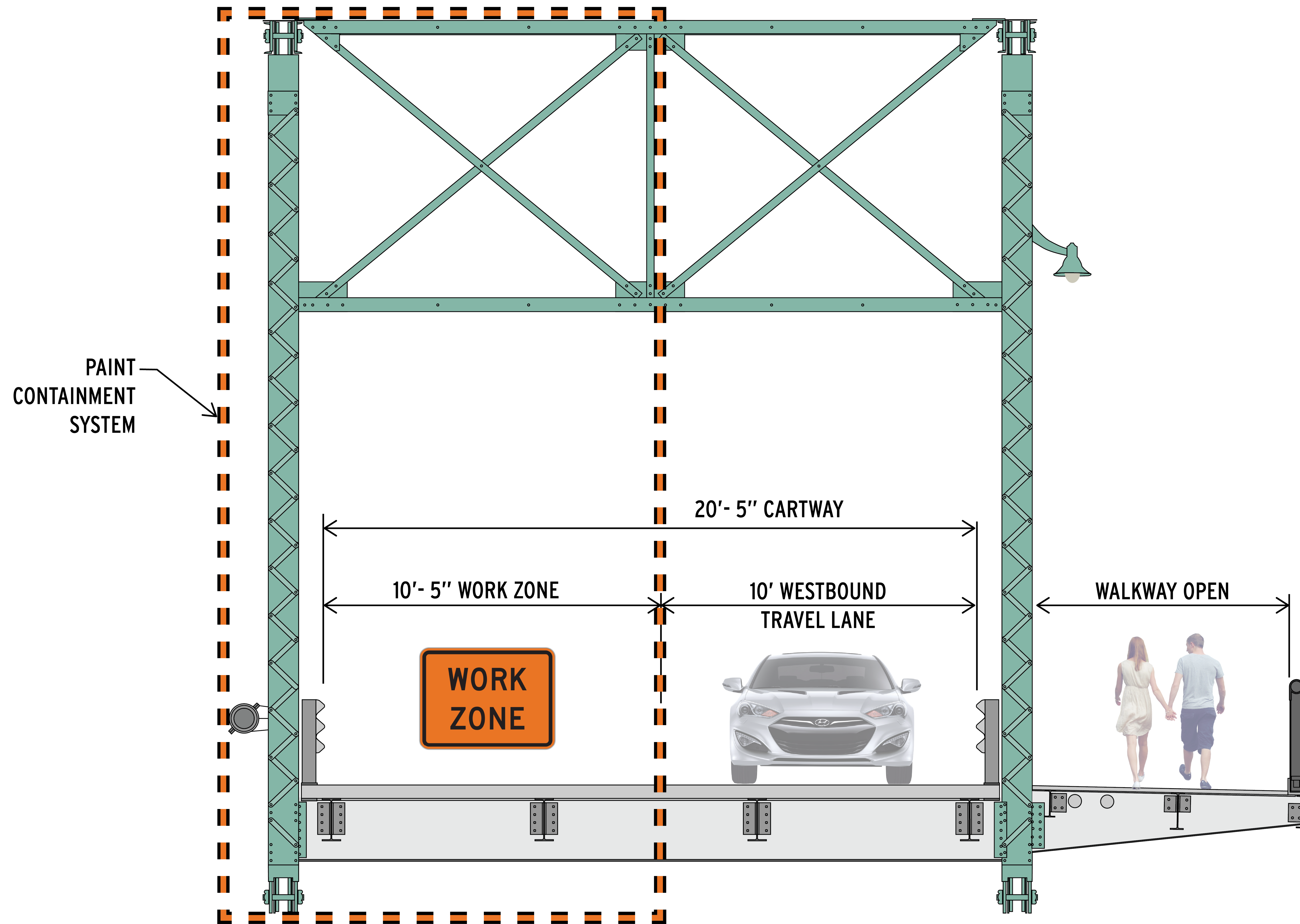
STAGE 1 - PORTION OF BRIDGE CLOSED (LOOKING EAST)
