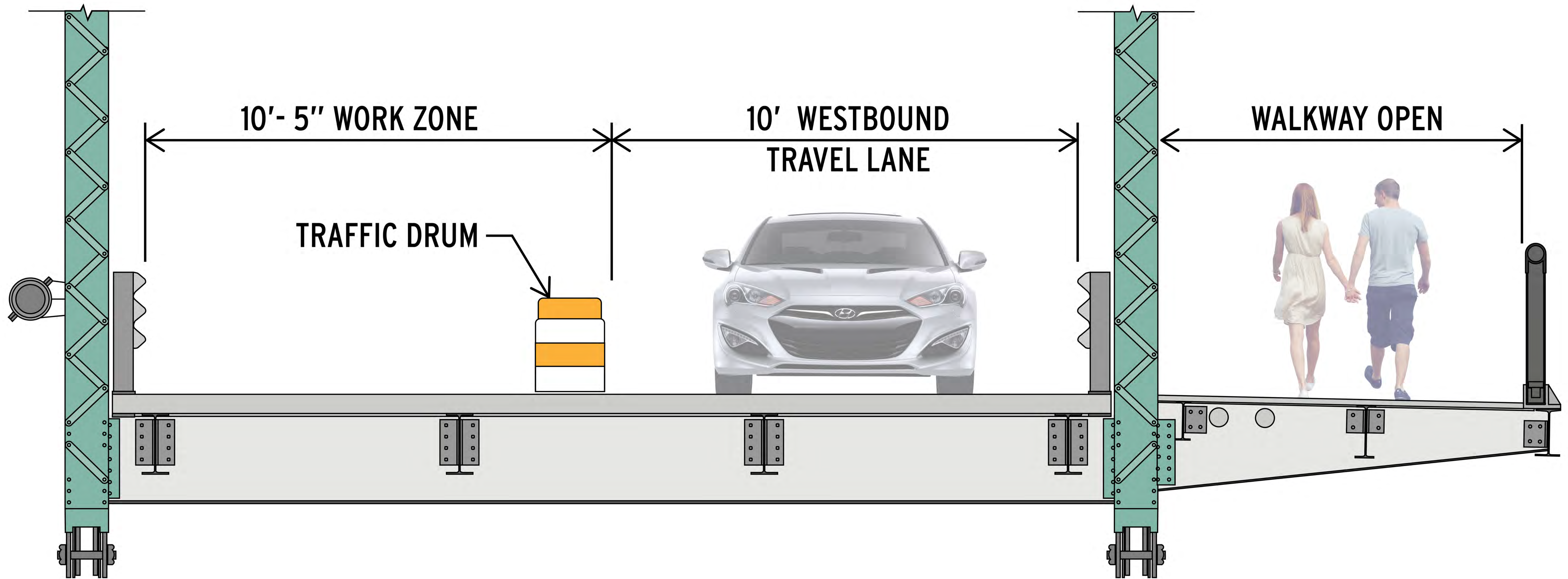
STAGE 3 - PORTION OF BRIDGE CLOSED MONDAY THROUGH FRIDAY (LOOKING EAST)
