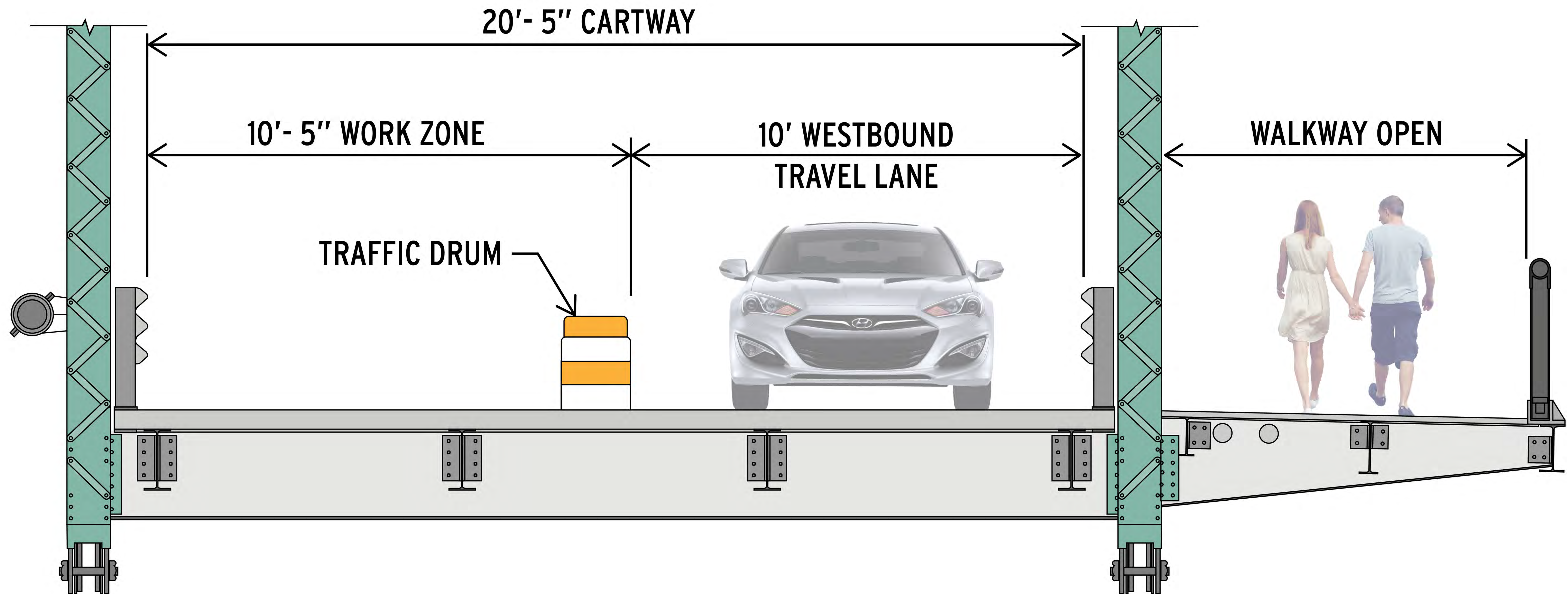
STAGE 2 - PORTION OF BRIDGE CLOSED (LOOKING EAST)
