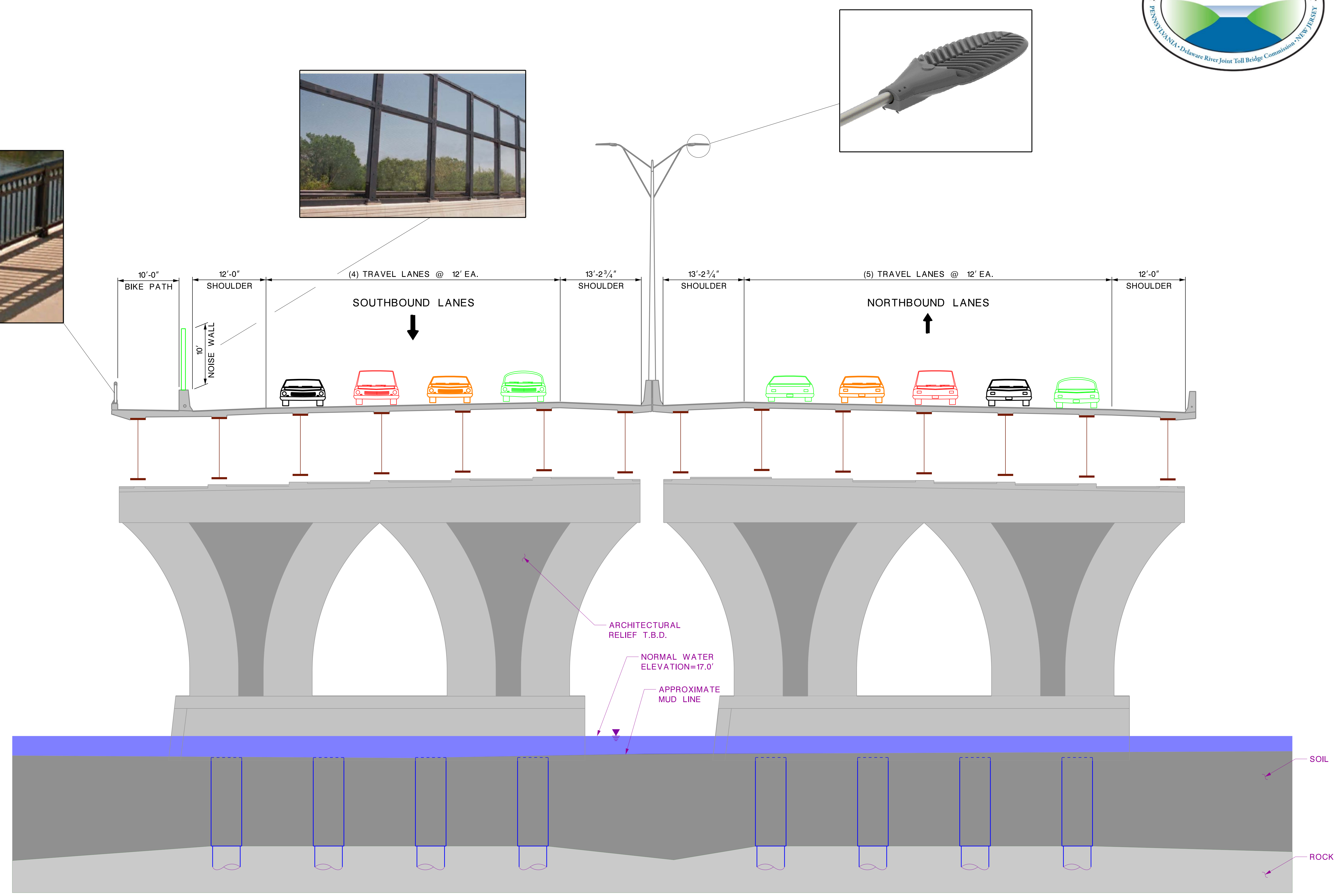
TYPICAL SECTION (LOOKING EAST)
