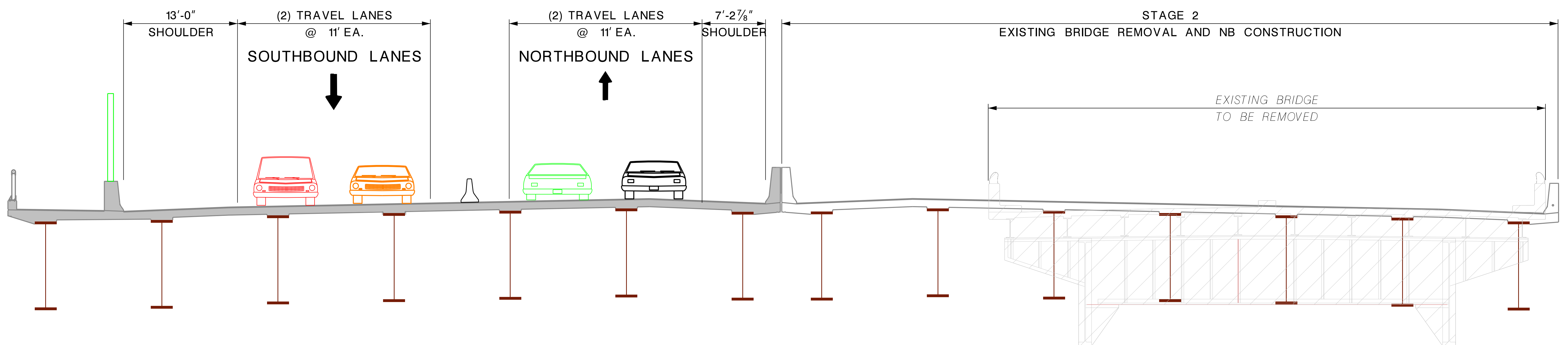
STAGE 2 - TRAFFIC, DEMOLITION AND NB CONSTRUCTION
