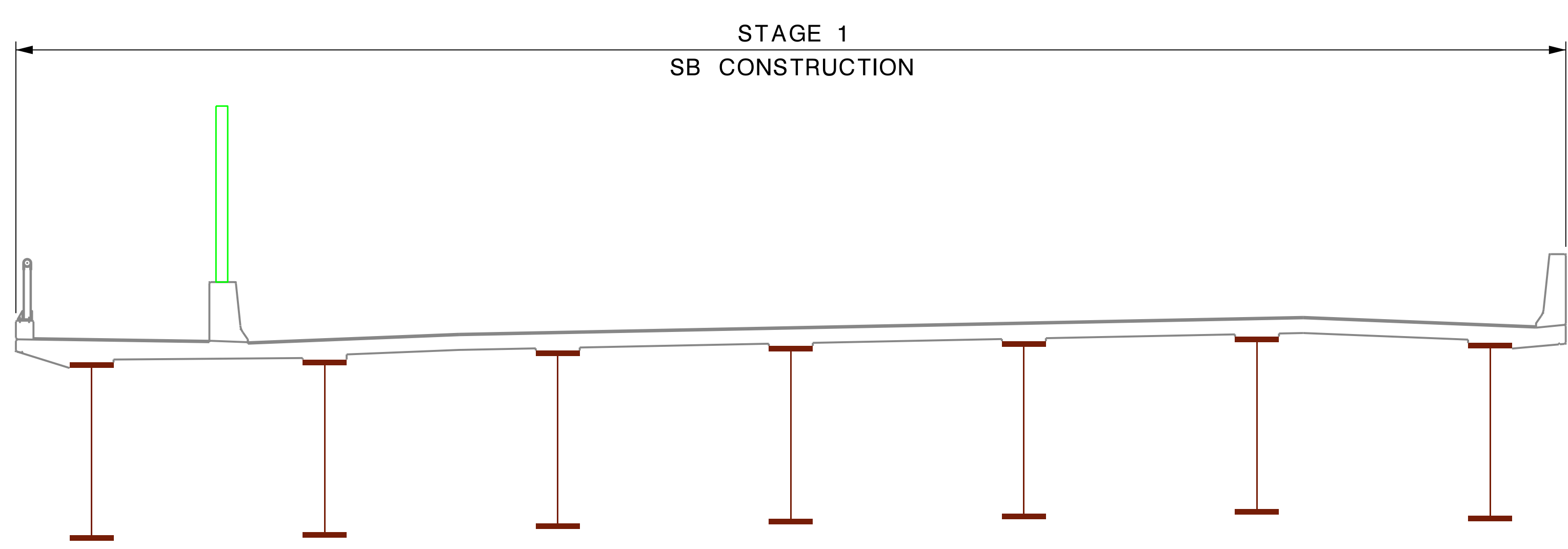
STAGE 1 - TRAFFIC AND SB CONSTRUCTION
