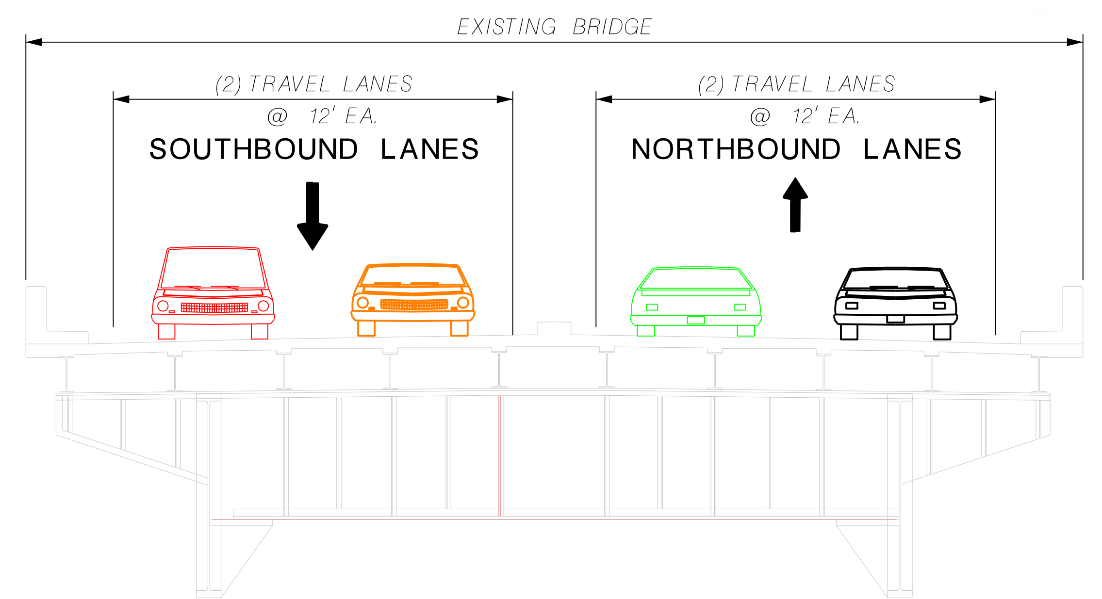
STAGE 1 - TRAFFIC AND SB CONSTRUCTION
